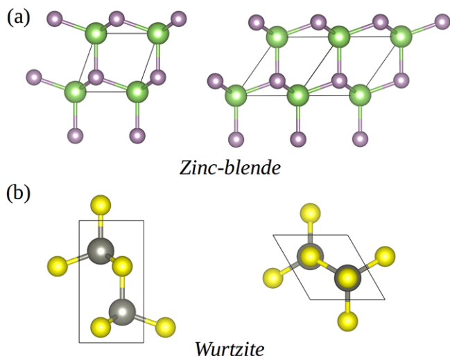
Figure 1. Polymorphism of bulk GaP and ZnS. a) The zinc-blende structure with space group F\bar{4}3m and cubic symmetry. b) The wurtzite structure with space group P6_3mc and hexagonal symmetry. Ga and Zn atoms are represented with green and black spheres and P and S atoms with purple and yellow spheres, respectively. In both structures, the ions are fourfold coordinated.
