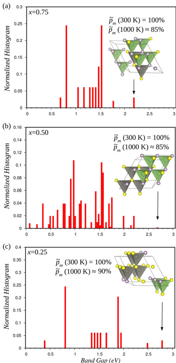
Figure 5. Normalized E_{\text{gap}} histogram for zinc-blende (\text{GaP})_x(\text{ZnS})_{1-x} solid solutions. a) x = 75\% , b) 50\% , and c) 25\% compositions. The histogram is constructed by dividing the number of structures within each specific band gap energy interval by the total number of structures. The inequivalent configuration that is most probable in each case is sketched along with its occurrence probability and energy band gap (black arrow). Ga and Zn atoms are represented with green and black spheres and P and S atoms with purple and yellow spheres, respectively. Energy band gaps are estimated with the HSE06 hybrid functional. [28]
