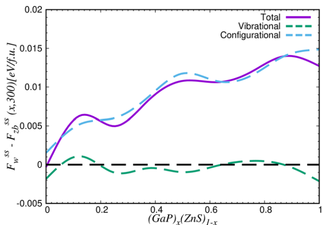
Figure 4. Free-energy difference between the two polymorphs for (\text{GaP})_x(\text{ZnS})_{1-x} solid solutions at T = 300 K. Zinc-blende and wurtzite phases are represented as “zb” and “w”, respectively. Configurational and vibrational contributions to the total free-energy difference are indicated. Note that for the end-members F_{\text{conf}} reduces to the static energy (see Equations (2) and (3)).
