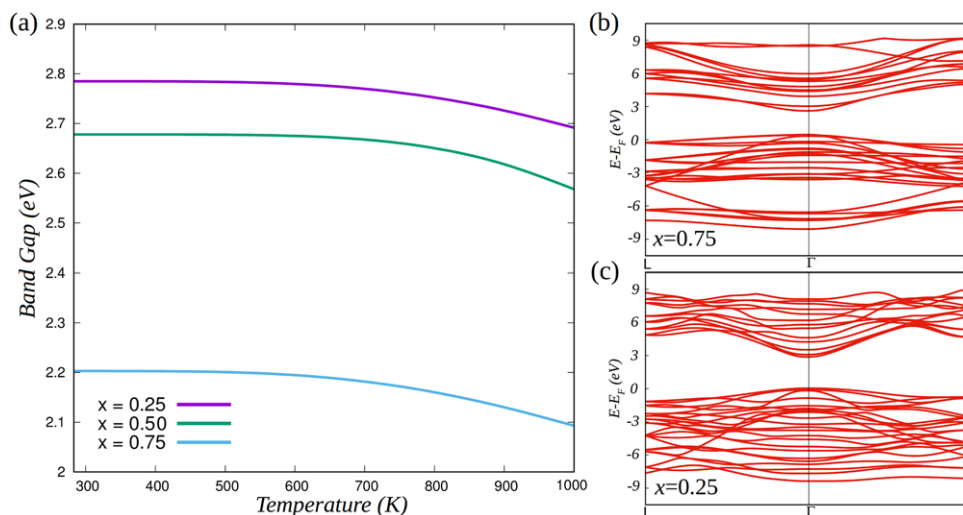
Figure 6. Electronic band structure of zinc-blende (\text{GaP})_x(\text{ZnS})_{1-x} solid solutions. a) Averaged energy band gap as a function of temperature and composition calculated with the multi-configurational supercell method. b) Electronic band structure calculated for the most probable configuration at x = 75\% , which renders a direct energy band gap at \Gamma . c) Idem at x = 25\% . Energy band gaps are estimated with the exchange-correlation HSE06 hybrid functional. [28]
