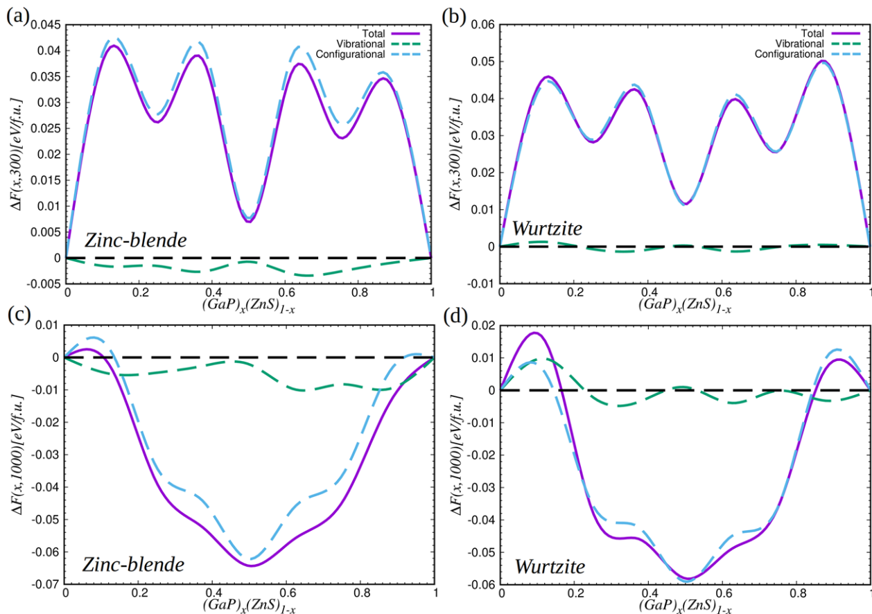
Figure 3. Mixing free-energy of (\text{GaP})_x(\text{ZnS})_{1-x} solid solutions at 300 and 1000 K. a–c) Zinc-blende and b–d) wurtzite structures. Vibrational and configurational (i.e., total minus vibrational) contributions to the total mixing free-energy of the system are expressed as a function of composition. Typical \Delta F errors are estimated to be of the order of 10 meV per formula unit.
