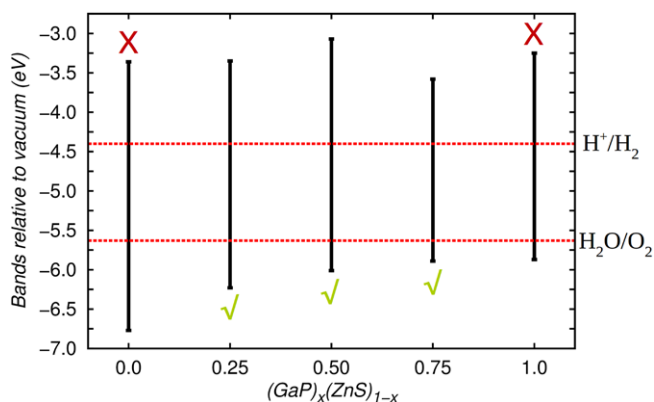
Figure 7. Energy bands relative to the vacuum level in zinc-blende (\text{GaP})_x(\text{ZnS})_{1-x} solid solutions. \Gamma energy band gaps are direct for compositions x = 0\% , 25\% , 50\% , and 75\% . All energy band gaps lie within the 2\text{--}3\text{ eV} interval except for ZnS. The redox potentials relative to the vacuum level for the hydrogen reduction and water oxidation reactions are indicated with dashed lines. Energy band gaps and levels are estimated with the B3PW hybrid functional [32] and CRYSTAL09 code. [31]
