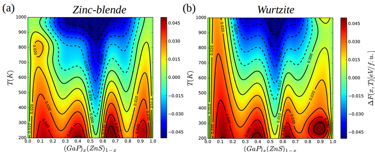
Figure 2. Mixing free-energy of (\text{GaP})_x(\text{ZnS})_{1-x} solid solutions as a function of temperature and composition. a) Zinc-blende and b) wurtzite structures. Solid lines represent iso-value \Delta F contours expressed in units of eV per formula unit. Typical \Delta F errors are estimated to be of the order of 10 meV per formula unit.
